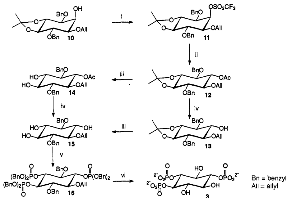
Scheme 1 Synthesis of DL- scyllo -inositol 1,2,4-trisphosphate 3 . Reagents and conditions : (i) triflic anhydride, pyridine, CH 2 Cl 2 , -78 °C; (ii) caesium acetate, dry DMF; (iii) M HCl, MeOH, reflux; (iv) M NaOH, MeOH, reflux; (v) (a) Pr i 2 NP(OBn) 2 , tetrazole, CH 2 Cl 2 ; (b) 70% tert -BuOOH; (vi) (a) Na-liq. NH 3 ; (b) water.
