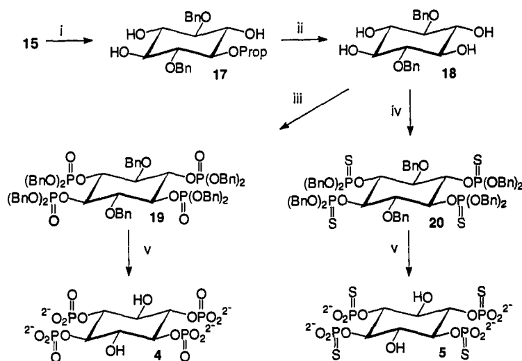
Scheme 2 Synthesis of scyllo -inositol 1,2,4,5-tetrakisphosphate 4 and scyllo -inositol 1,2,4,5-tetrakisphosphorothioate 5 . Reagents and conditions: (i) \text{KOBu}^t , DMSO, 50 °C; (ii) \text{M HCl} , MeOH, reflux; (iii) (a) \text{Pr}_2\text{NP}(\text{OBn})_2 , tetrazole, \text{CH}_2\text{Cl}_2 ; (b) 70% tert -BuOOH; (iv) (a) \text{Pr}_2\text{NP}(\text{OBn})_2 , tetrazole, \text{CH}_2\text{Cl}_2 ; (b) \text{S}_8 , pyridine; (v) (a) \text{Na} -liq. \text{NH}_3 ; (b) water.
