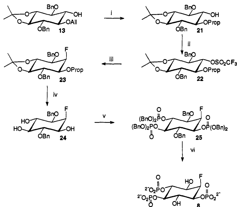
Scheme 3 Synthesis of DL-2-deoxy-2-fluoro-Ins(1,4,5) P_3 8 . Reagents and conditions: (i) \text{KOBu}^t , DMSO, 50 °C; (ii) trific anhydride, pyridine, \text{CH}_2\text{Cl}_2 , -78 °C; (iii) TBAF, THF; (iv) M HCl, MeOH, reflux; (v) (a) \text{Pr}^t_2\text{NP}(\text{OBn})_2 , tetrazole, \text{CH}_2\text{Cl}_2 ; (b) 70% tert -BuOOH; (vi) (a) Na-liq. \text{NH}_3 ; (b) water.
